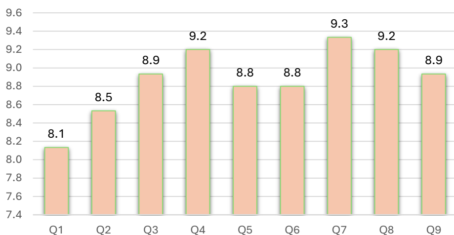
Differential Equations
