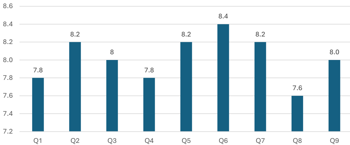
Software Engineering
