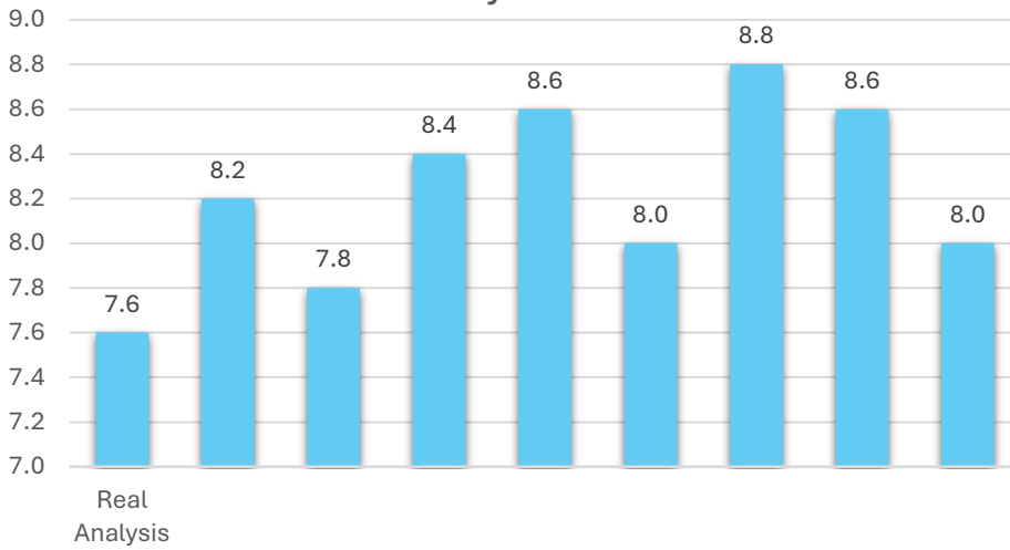
Real Analysis
